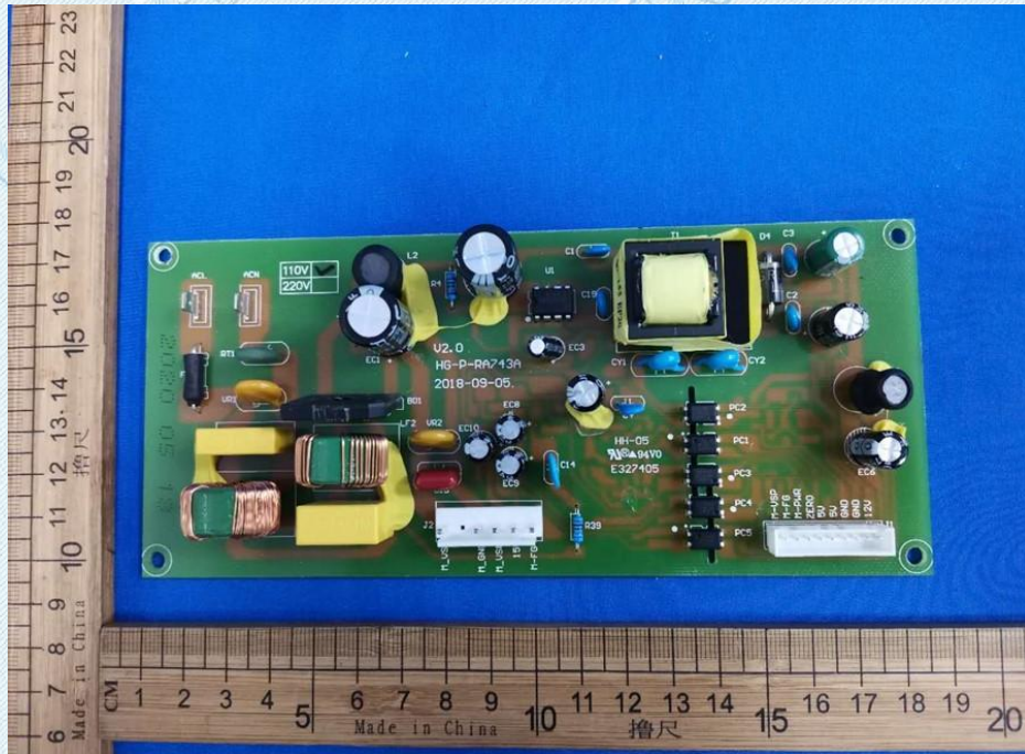
Photo 9 - PCB view
