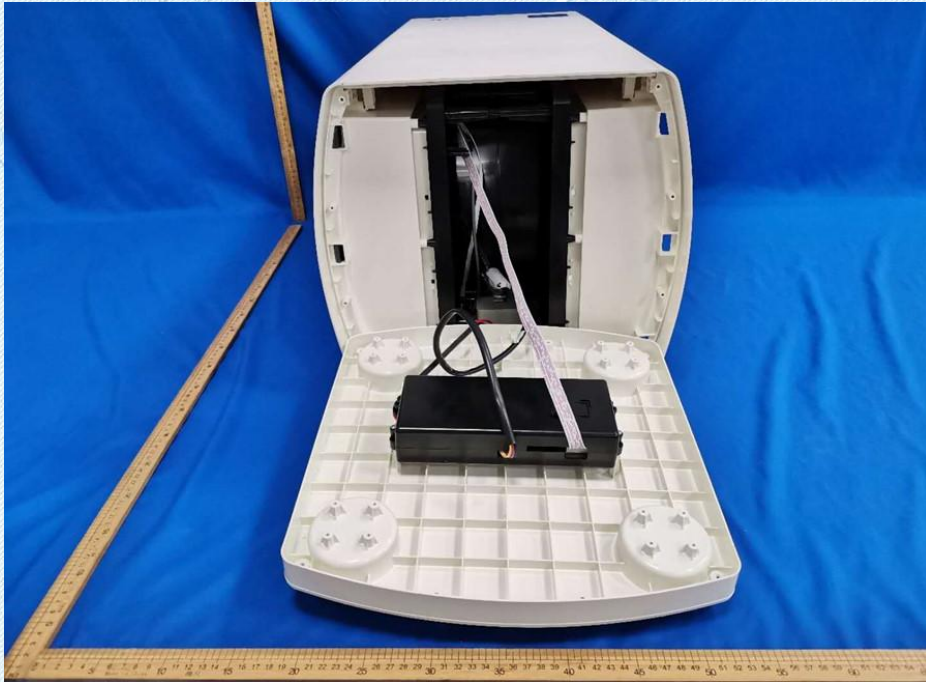
Photo 7 - Internal view
