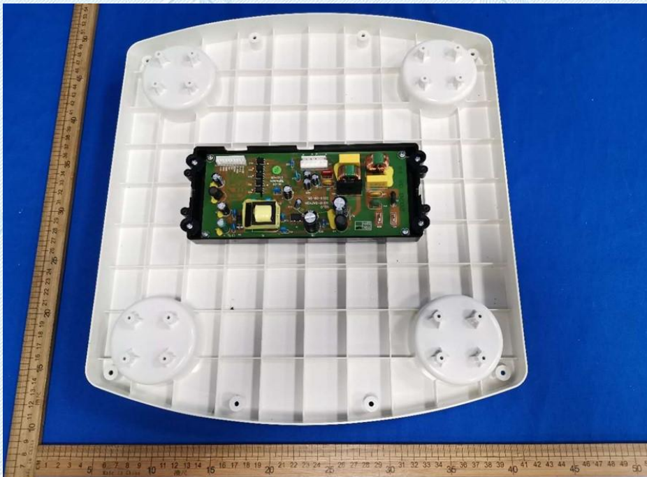
Photo 8 - Internal view
